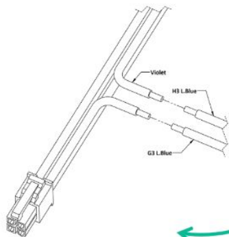
Brake Pedal connection
